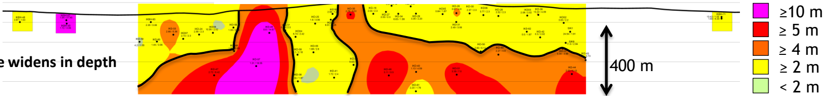
Grade contours
